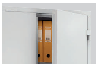
Double-wall construction filled with fire-resistant material
